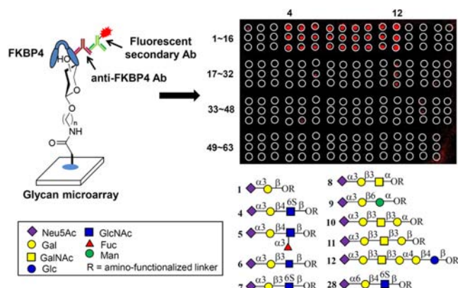
Figure 3. Binding analysis of FKBP4 in a printed glycan array with 63 glycans. Glycans (100 \mu\text{M} ) were printed in triplicate and probed with FKBP4 as described in the Supporting Information. The structures of FKBP4-binding glycans are shown.
