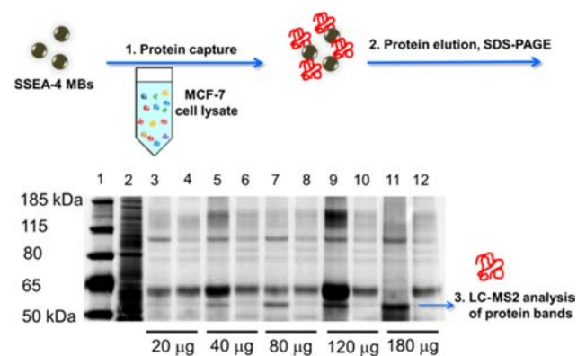
Figure 2. Magnetic bead-based capture for the identification of SSEA-4-binding proteins. Different amounts (20, 40, 80, 120, 180 \mu\text{g} ) of MCF-7 total cell lysate were mixed with SSEA-4-MBs or MEG-MBs (100 \mu\text{g} each), and the bound proteins were eluted, separated by SDS-PAGE, and visualized after silver staining. Lane 1, marker; lane 2, MCF-7 total cell lysate (0.5 \mu\text{g} ); lanes 3, 5, 7, 9, and 11, protein eluted from SSEA-4-MBs; lanes 4, 6, 8, 10, and 12, protein eluted from MEG-MBs for comparison.
