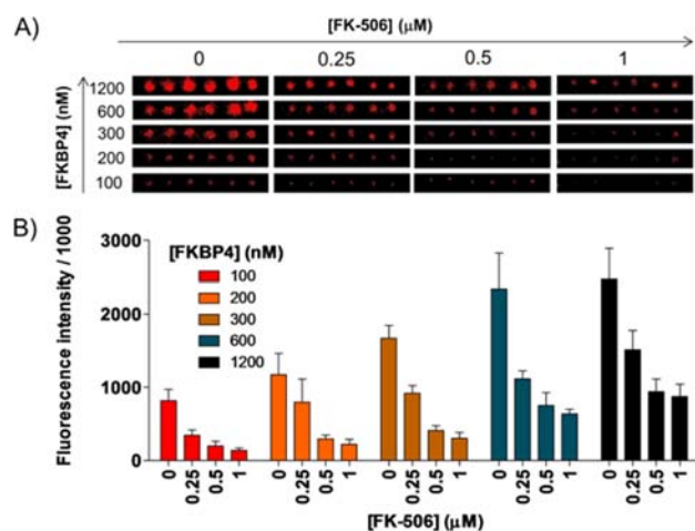
Figure 4. Competitive inhibition of SSEA-4/FKBP4 interaction by FK-506. Different concentrations of FKBP4 (100 nM to 1.2 \mu\text{M} ) and FK-506 (0–1 \mu\text{M} ) were tested in this competition assay. SSEA-4 (100 \mu\text{M} ) was printed with six replicates on the array. Glycan array images (A) and the relative geometric mean of fluorescence intensity (B) in each experimental set are shown.
